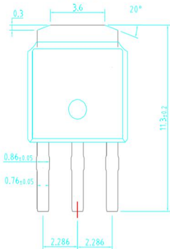
TO-251
