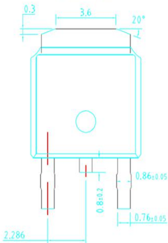
TO-252
